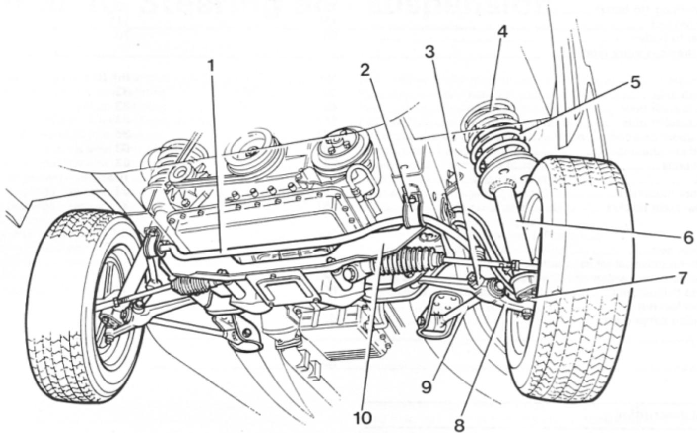
Fig. 10.2 Front suspension components (Sec 1)
