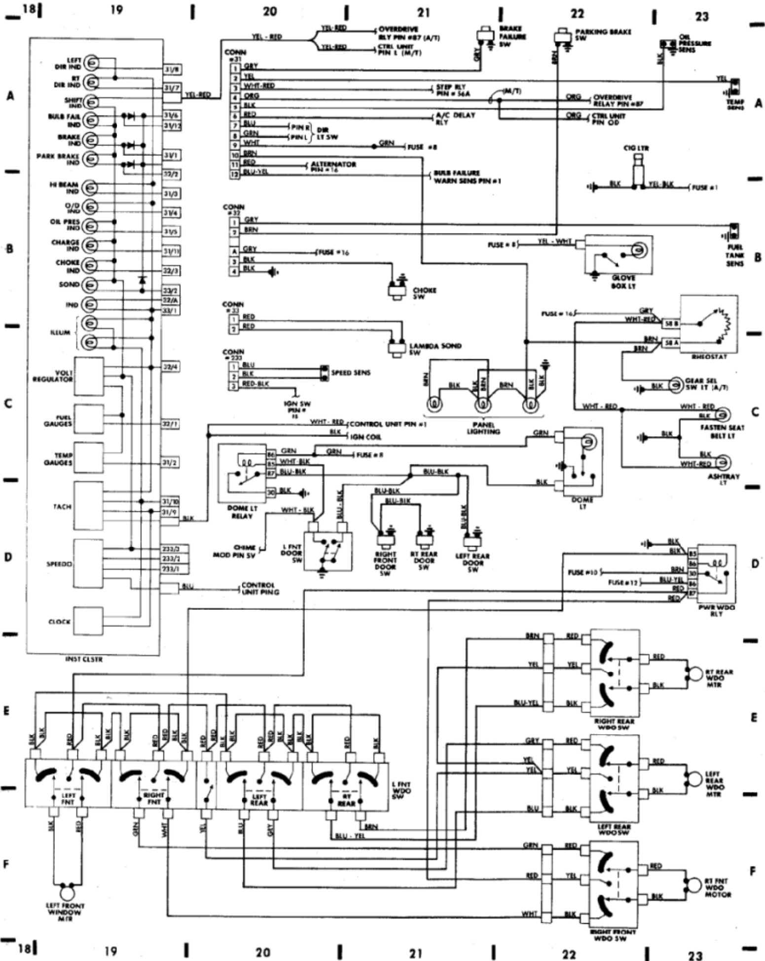
Fig. 5: Instrument Panel (Grids 18-23)
