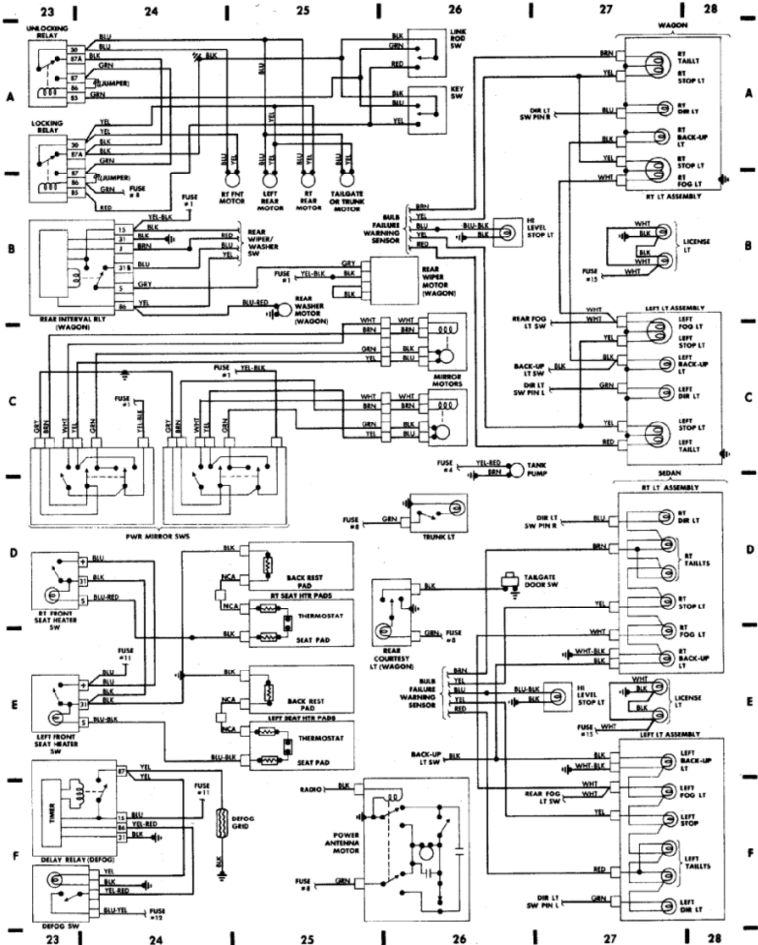
Fig. 6: Rear Compartment & Accessories (Grids 23-28)
