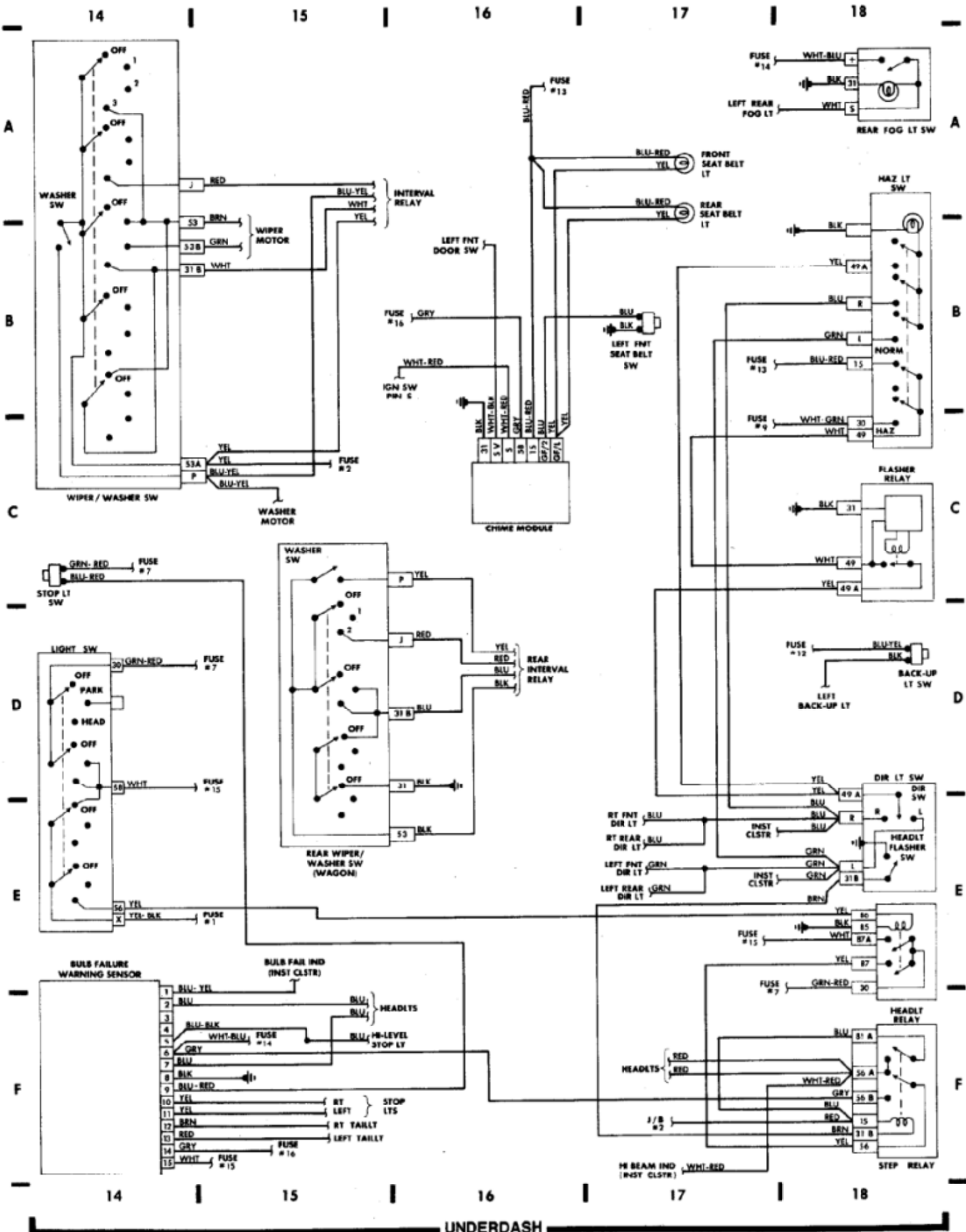
WIRING DIAGRAMS Fig. 4: Underdash (Grids 14-18) 1986 Volvo 240DL/GL
