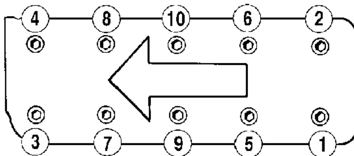
2.3L 4-CYL & 2.3L 4-CYL TURBO Fig. 3: Cylinder Head Bolt Removal & Installation Sequence
