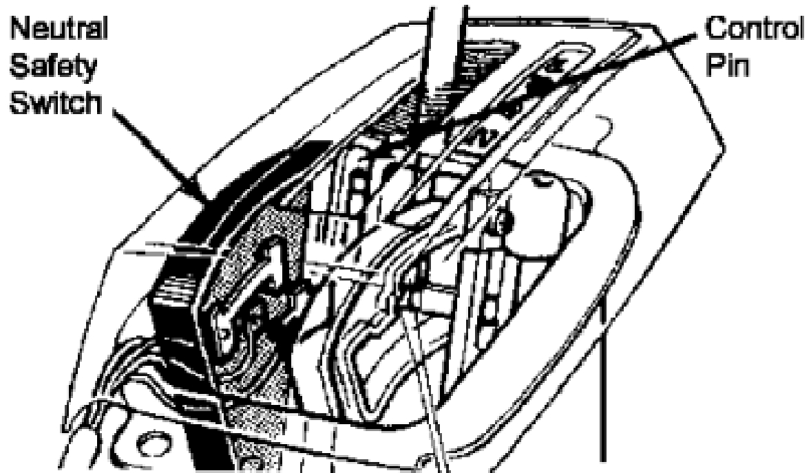
Fig. 4: Adjusting Neutral Safety Switch
