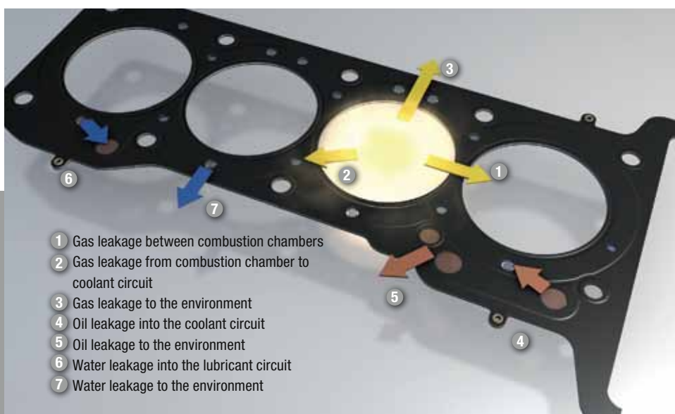
◀ Typical media leakages with MLS cylinder-head gaskets
