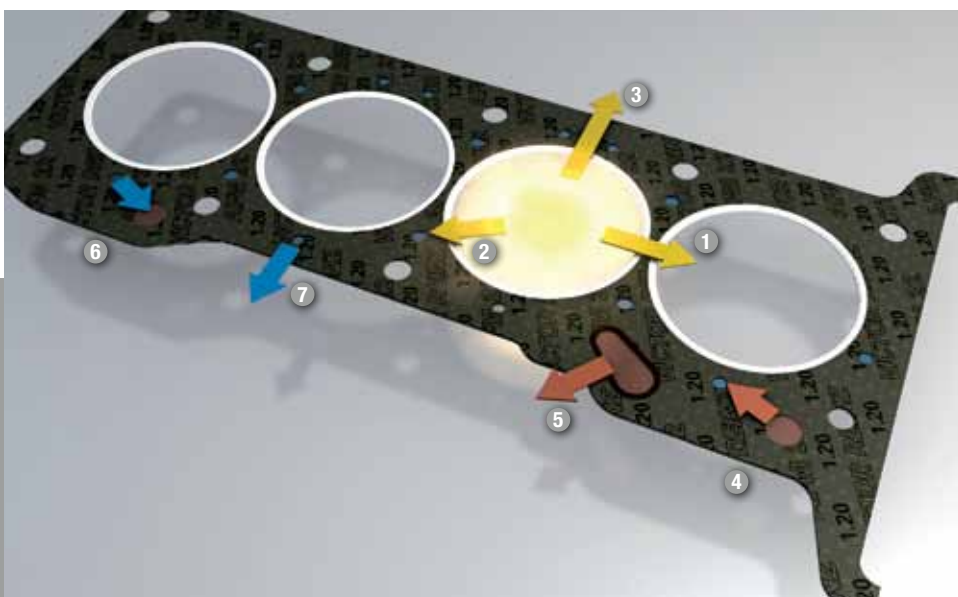
◀ Typical media leakages with composite cylinder-head gaskets.
