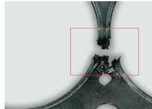
▲ Destruction in the web area due to combustion gas blowby.
