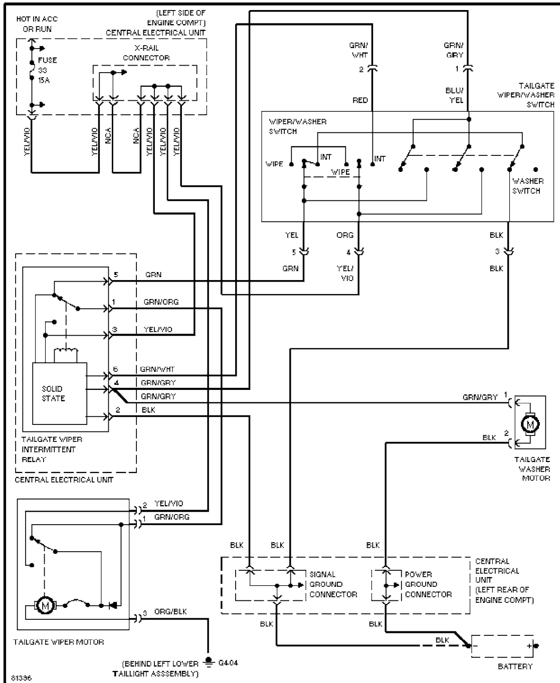
Rear Wiper/Washer Circuit, Late Production
