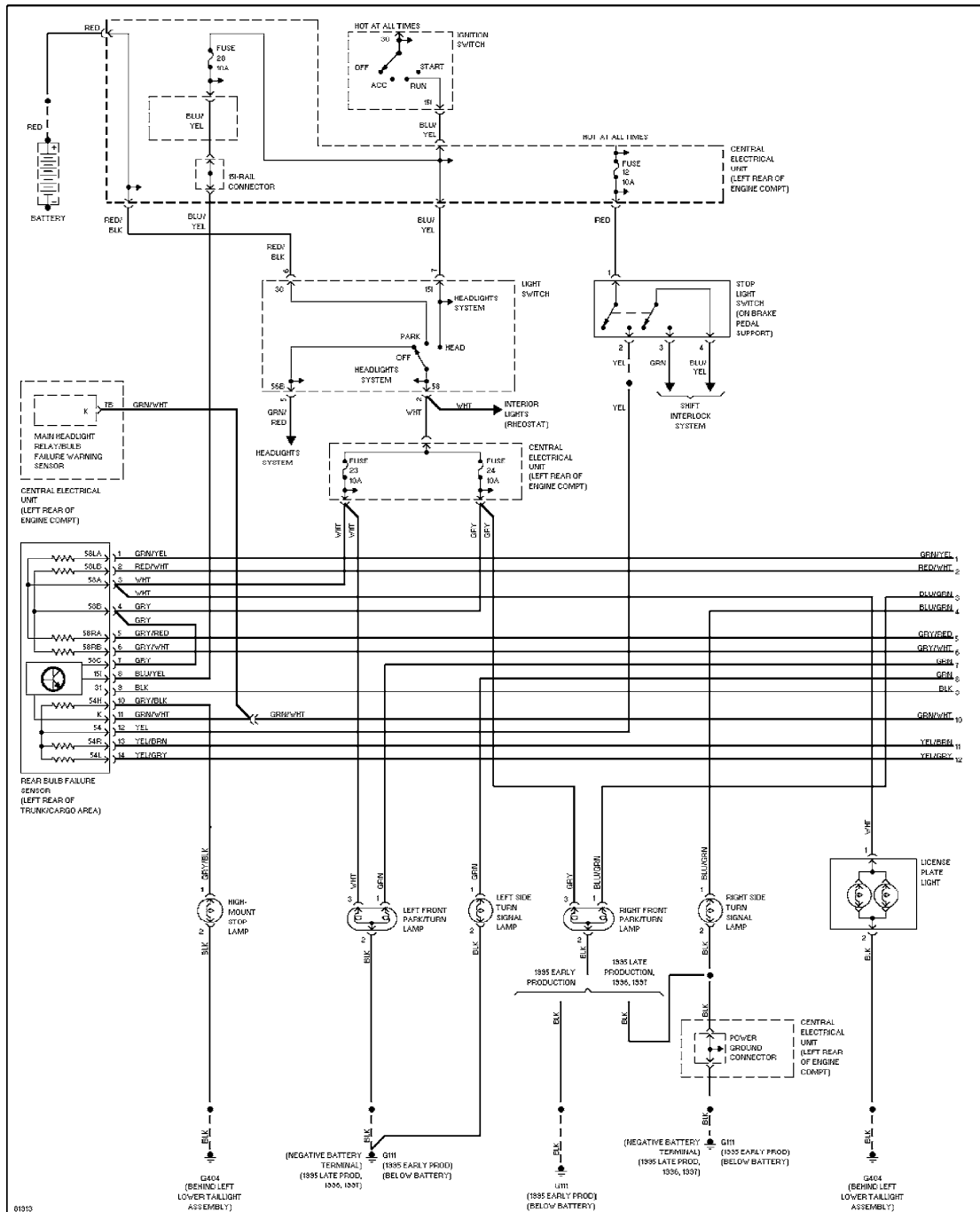
Exterior Lamps Circuit, Wagon (1 of 2)
