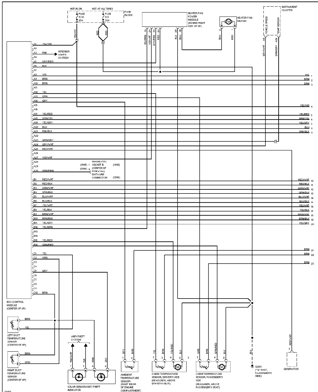
2.4L, Air Conditioning Circuits, Auto A/C (1 of 2)
