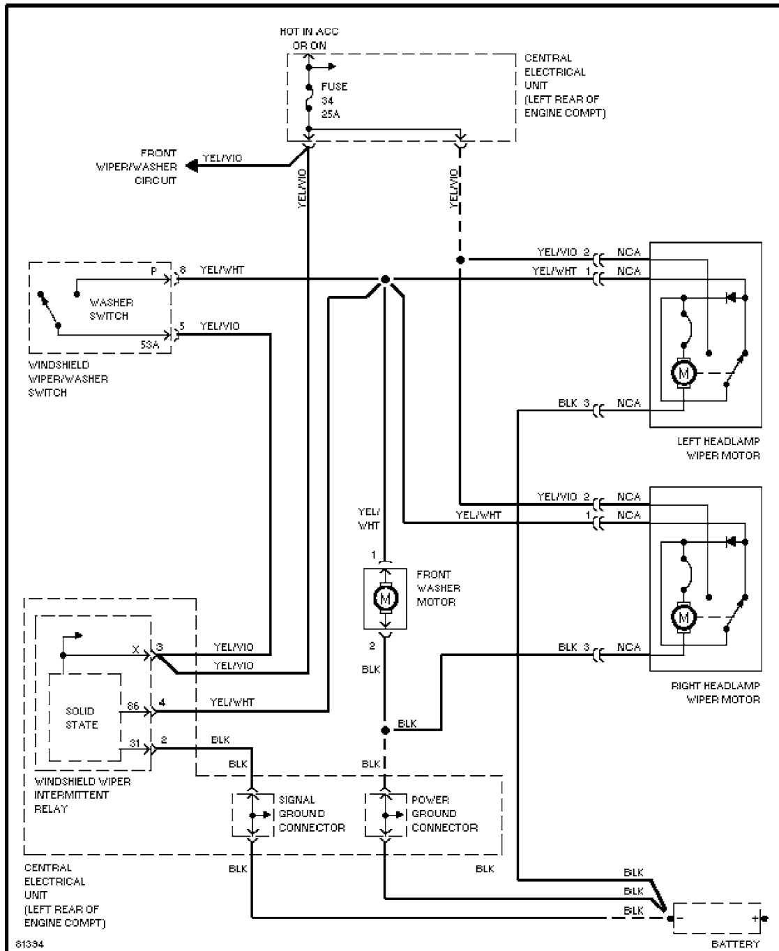
Headlamp Wiper/Washer Circuit, Late Production
