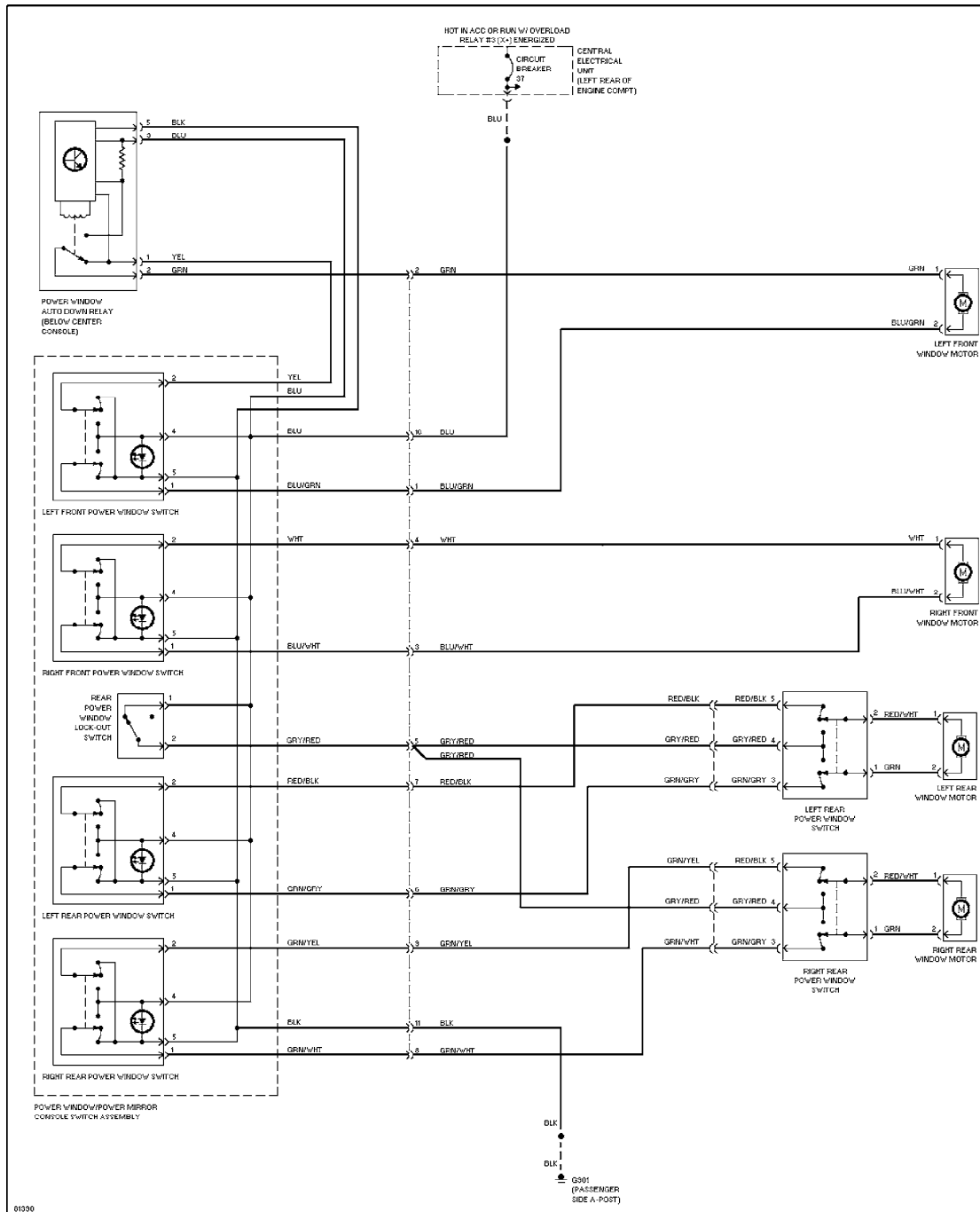
Power Window Circuit
