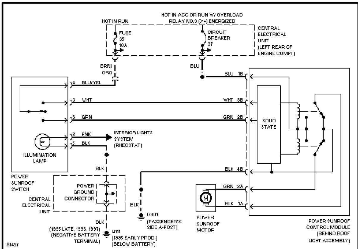
Power Top/Sunroof Circuits
