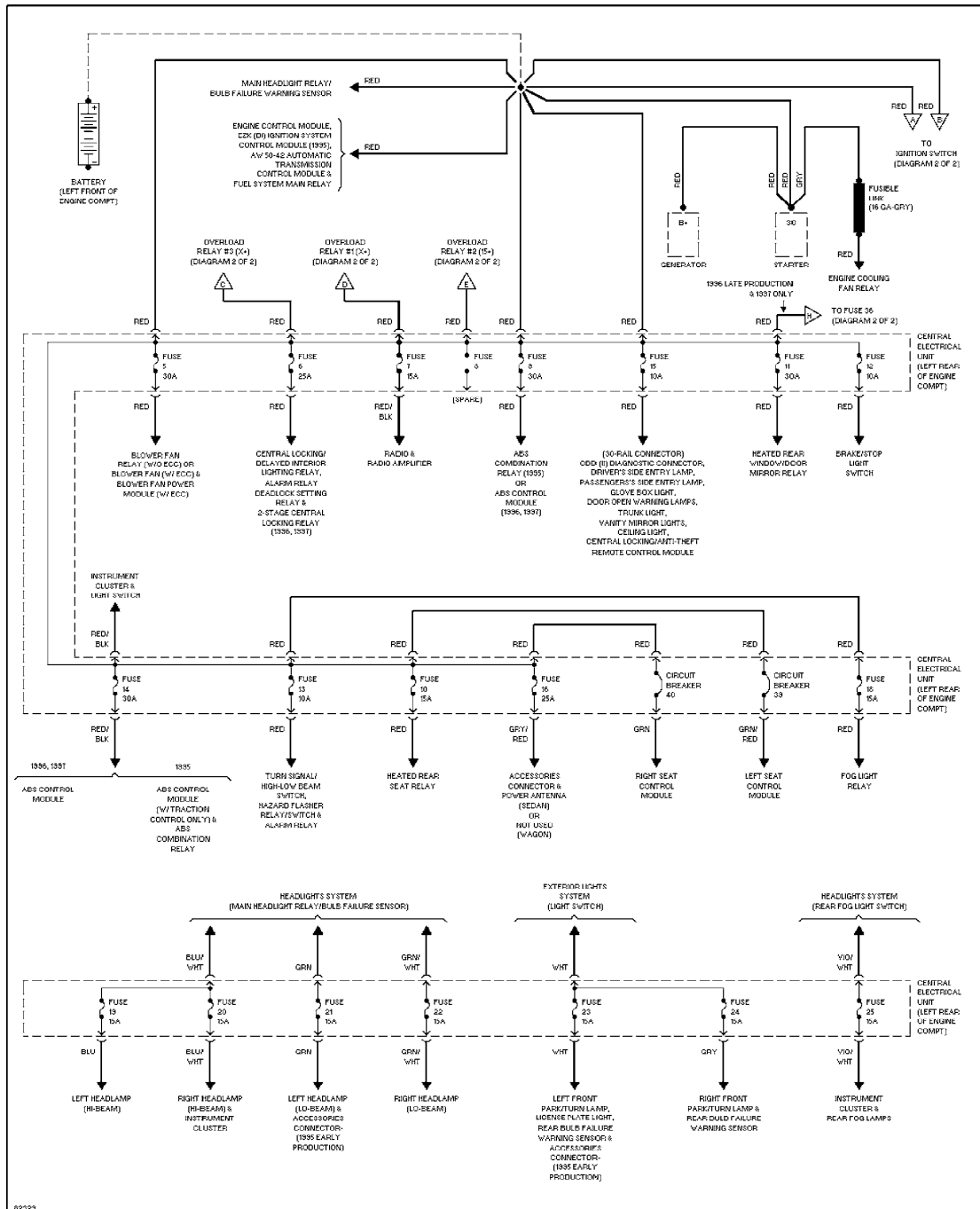
Power Distribution Circuit (1 of 2)
