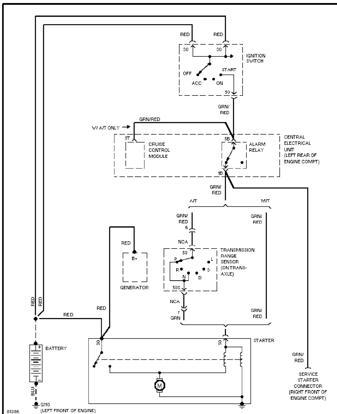
Starting Circuit
