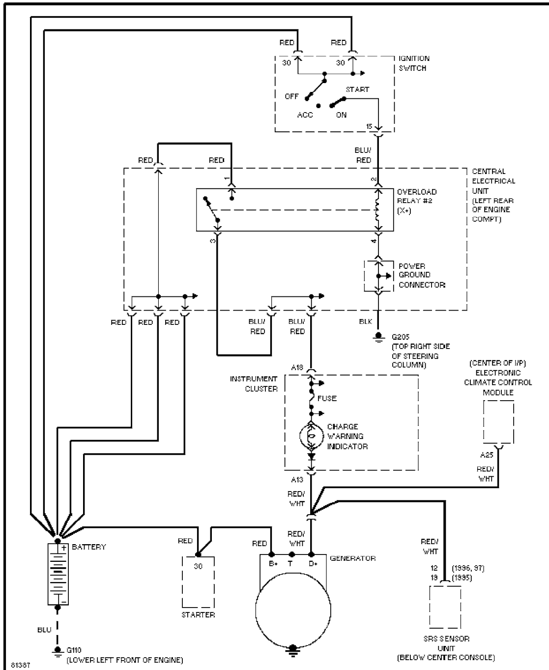
Charging Circuit
