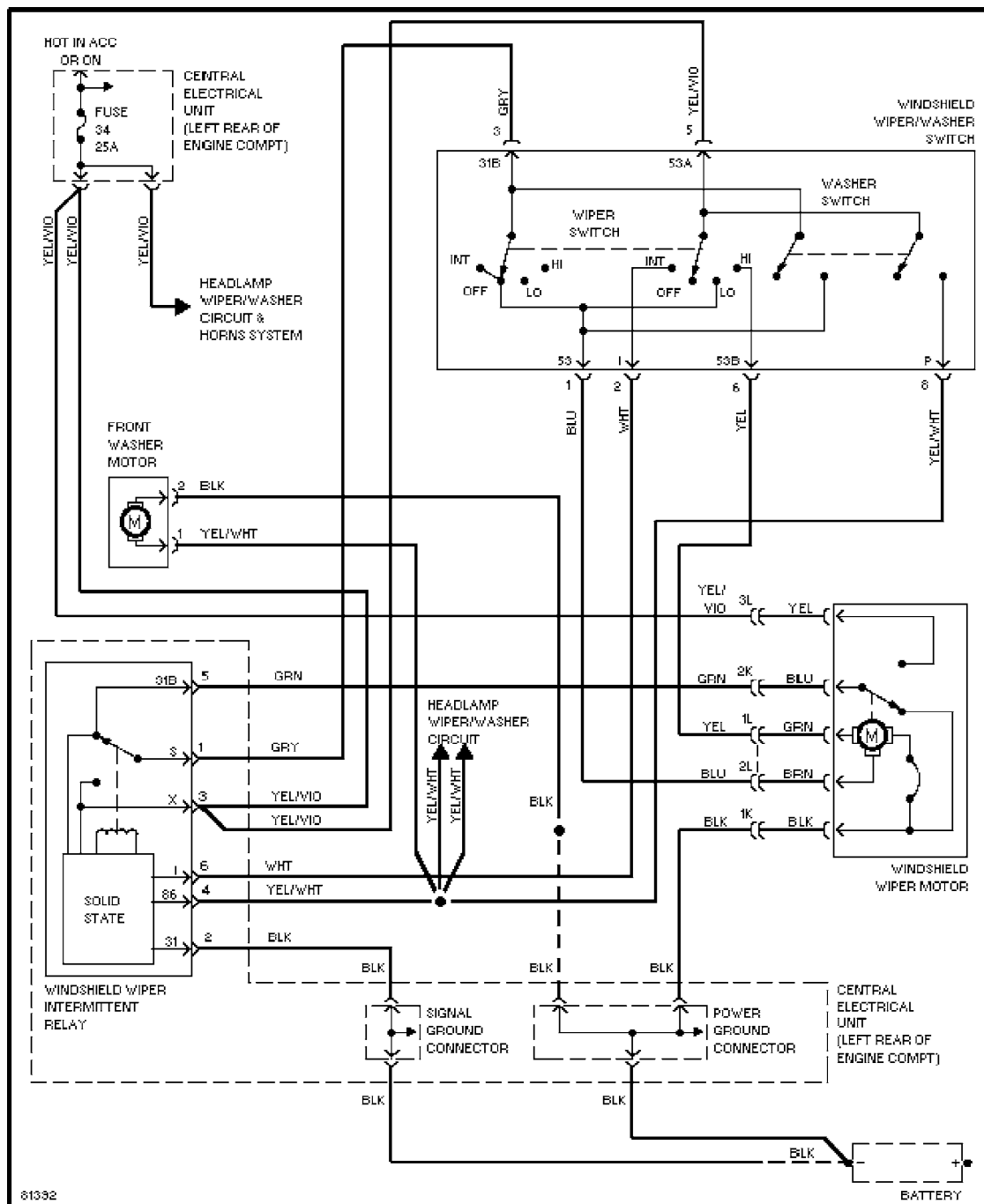
Front Wiper/Washer Circuit, Late Production
