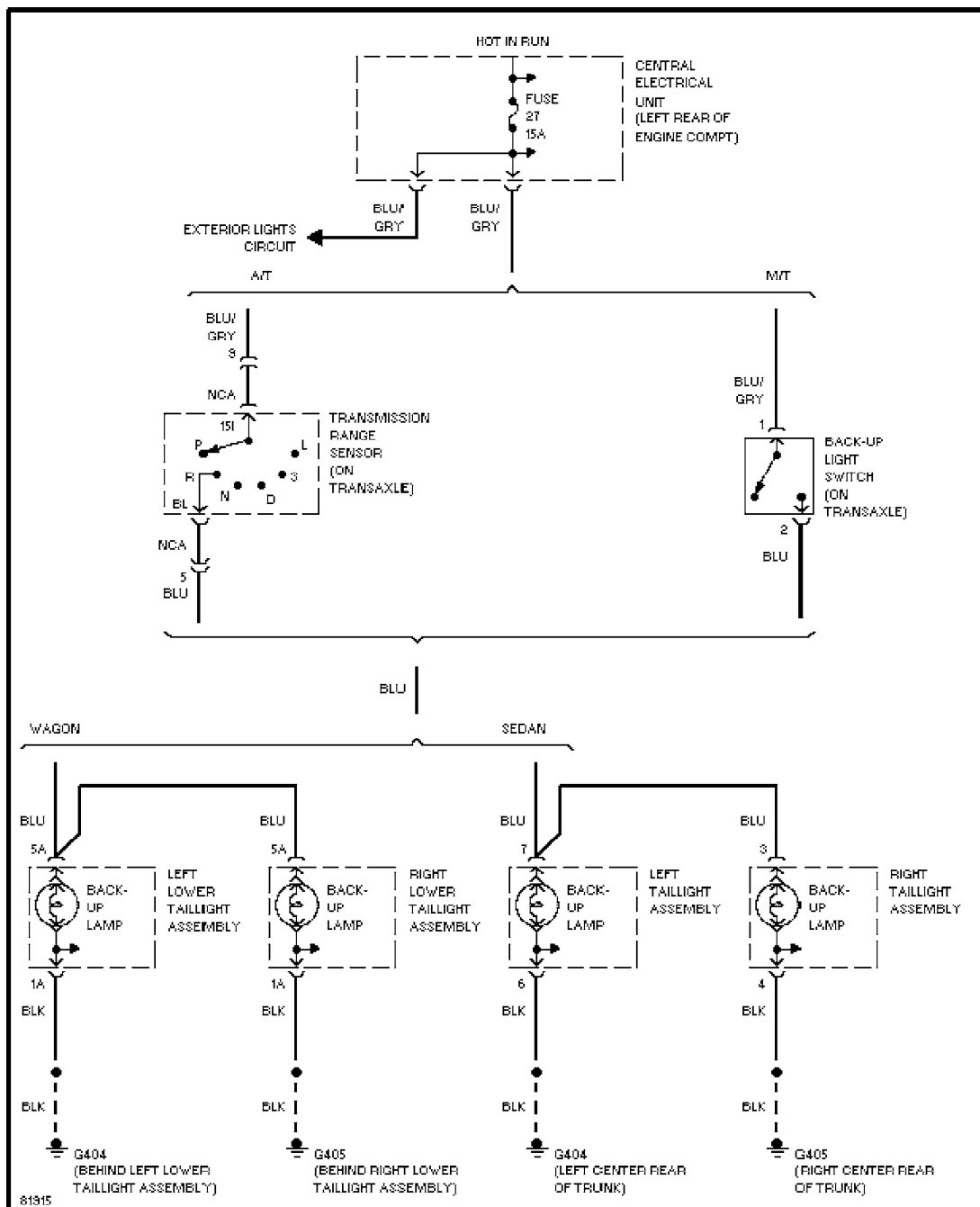
Back-up Lamps Circuit
