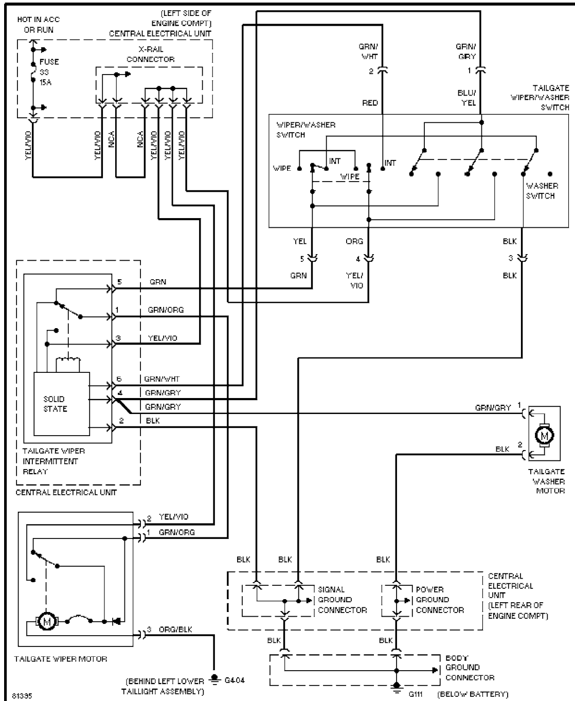
Rear Wiper/Washer Circuit, Early Production
