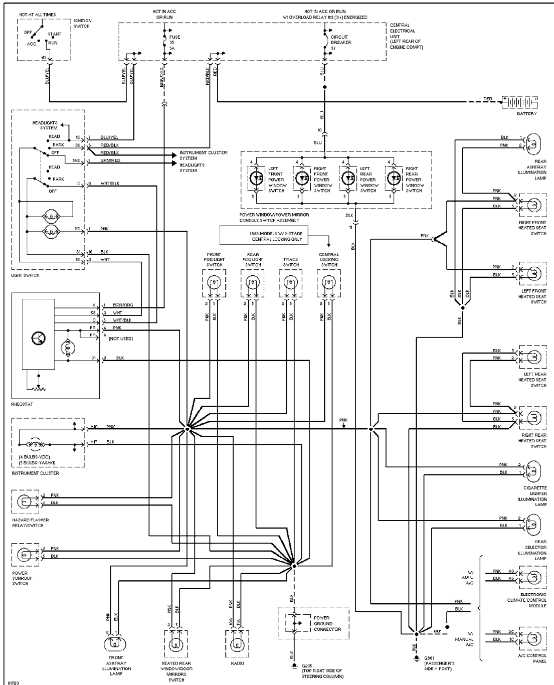
Instrument Illumination Circuit
