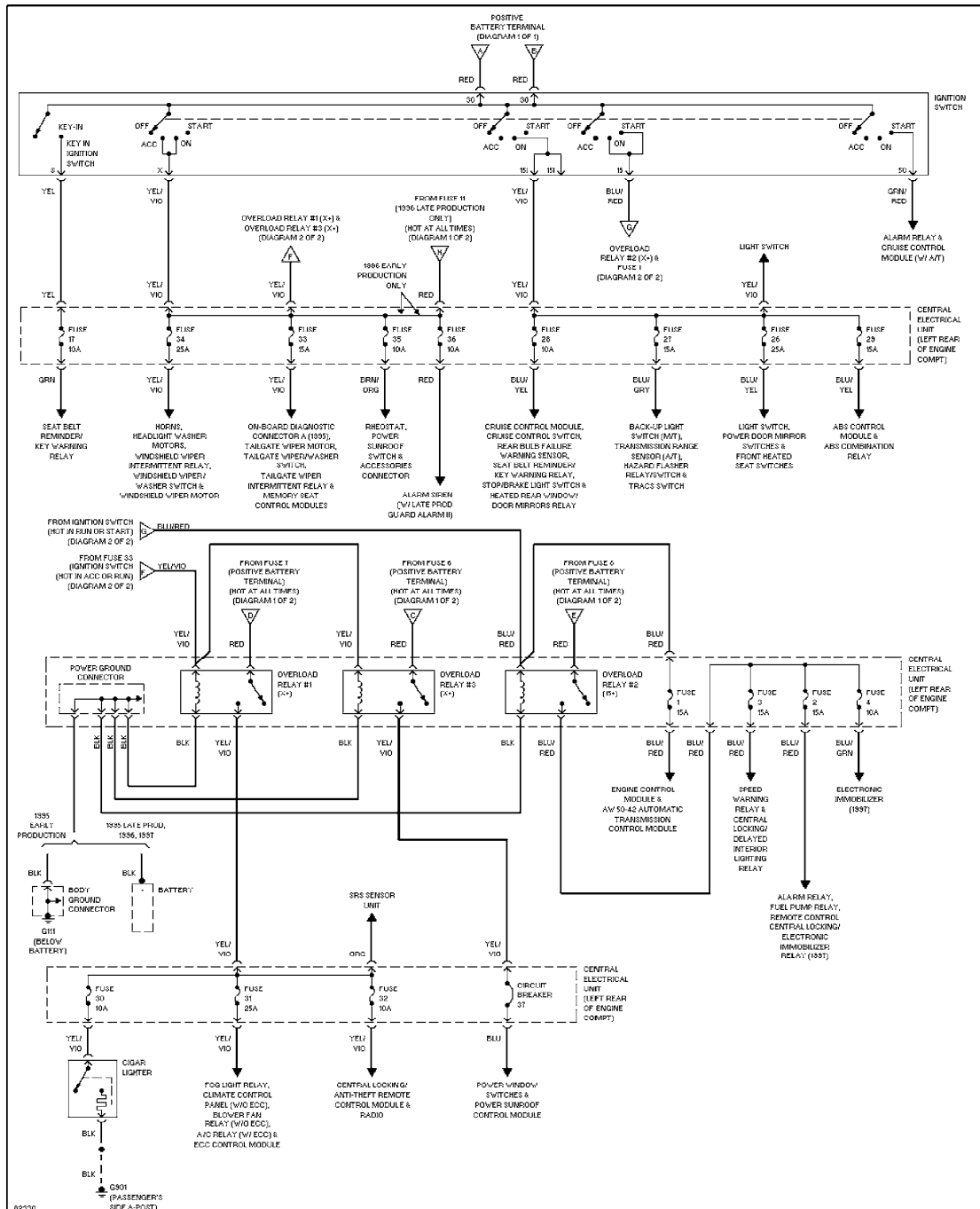
Power Distribution Circuit (2 of 2)
