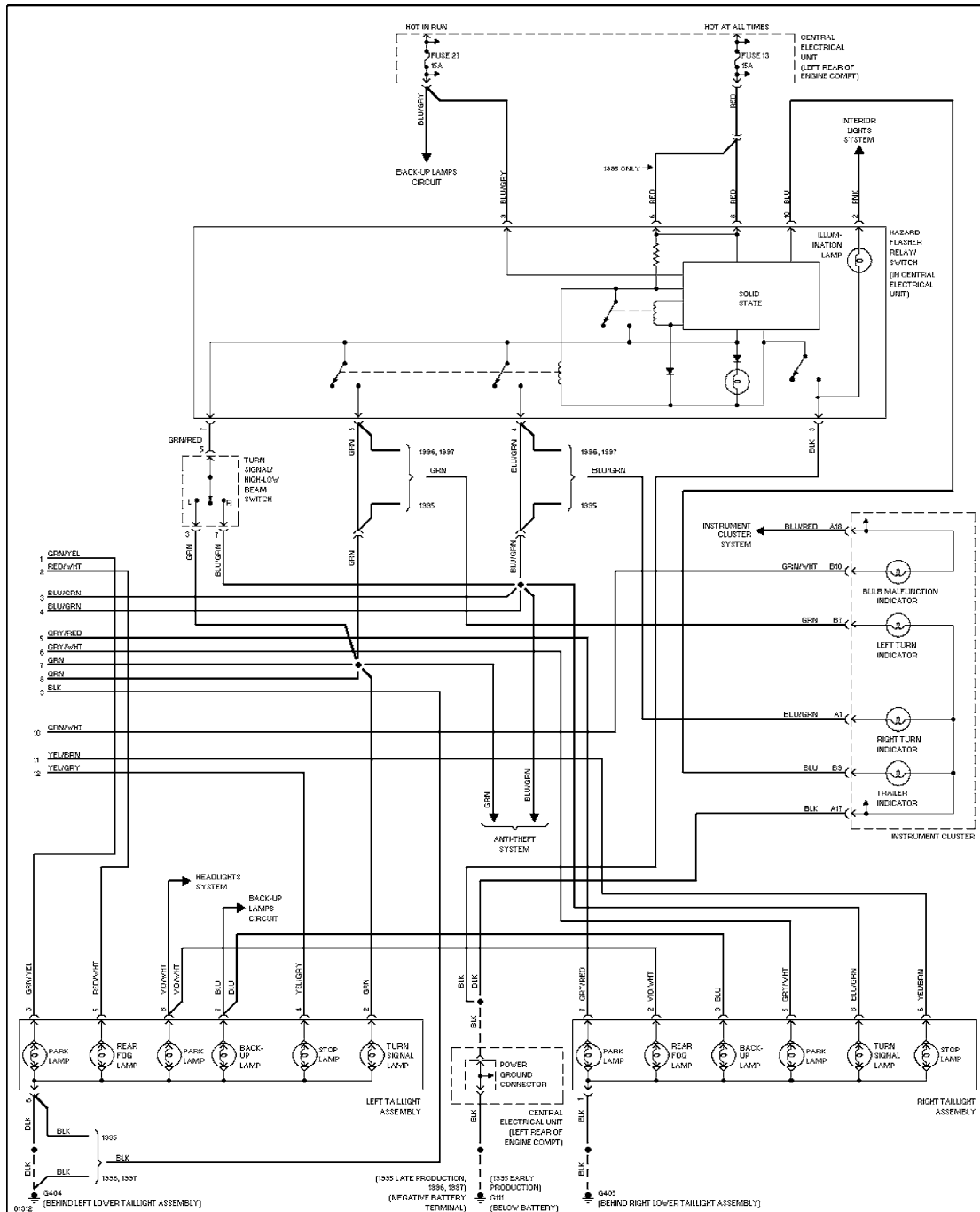
Exterior Lamps Circuit, Sedan (2 of 2)
