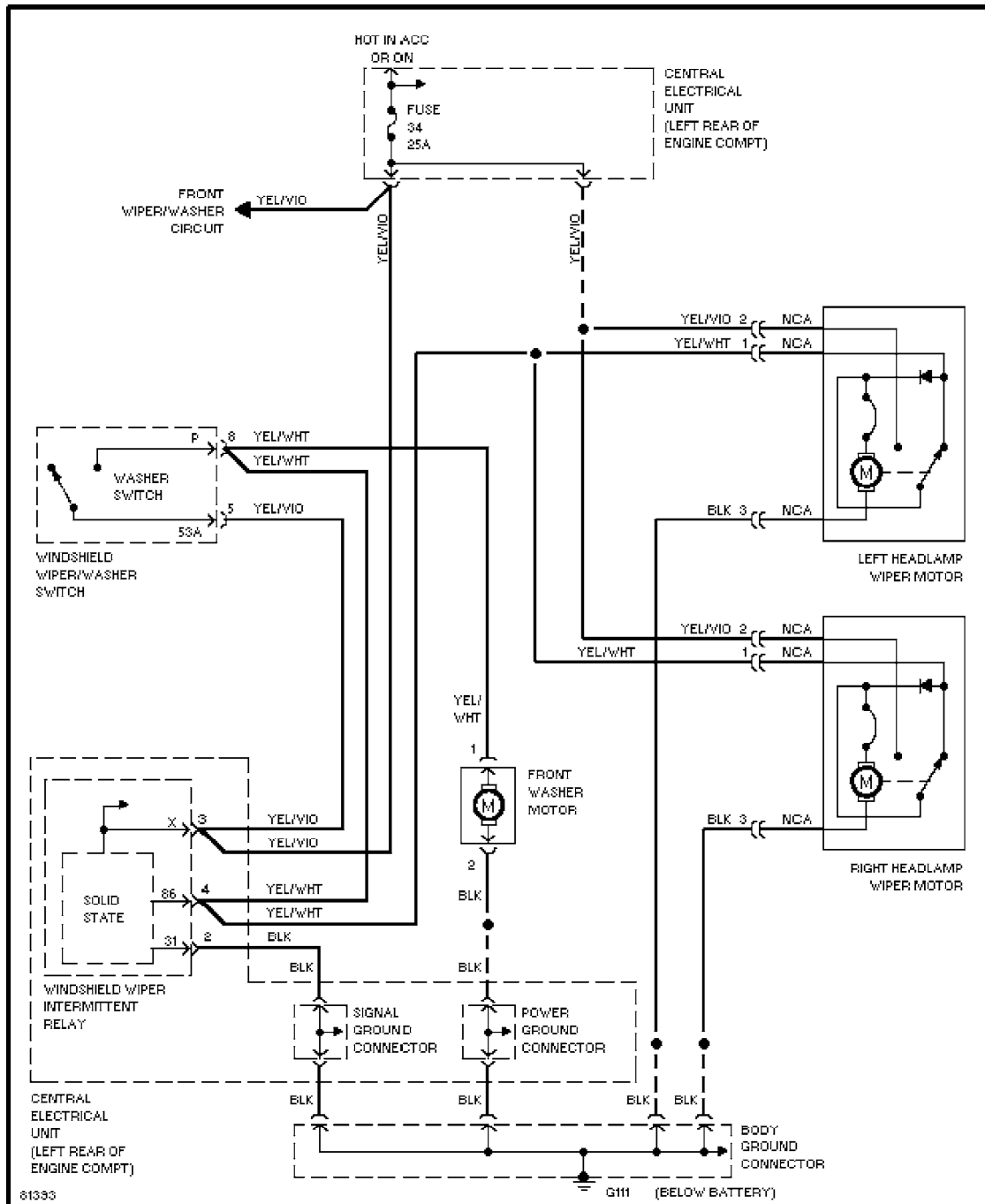
Headlamp Wiper/Washer Circuit, Early Production
