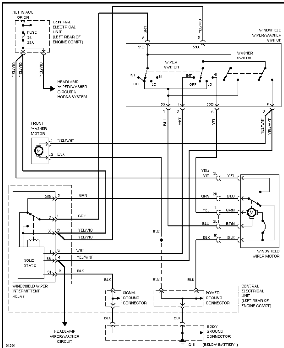
Front Wiper/Washer Circuit, Early Production
