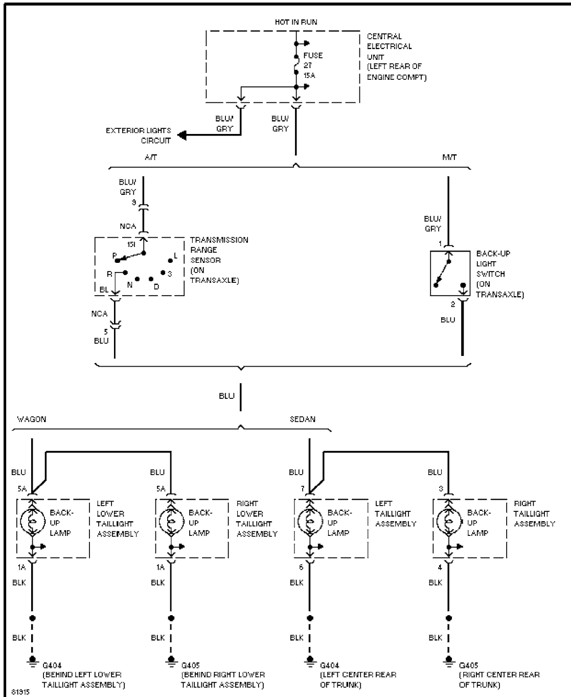
Backup Lamps Circuit, Sedan & Wagon
