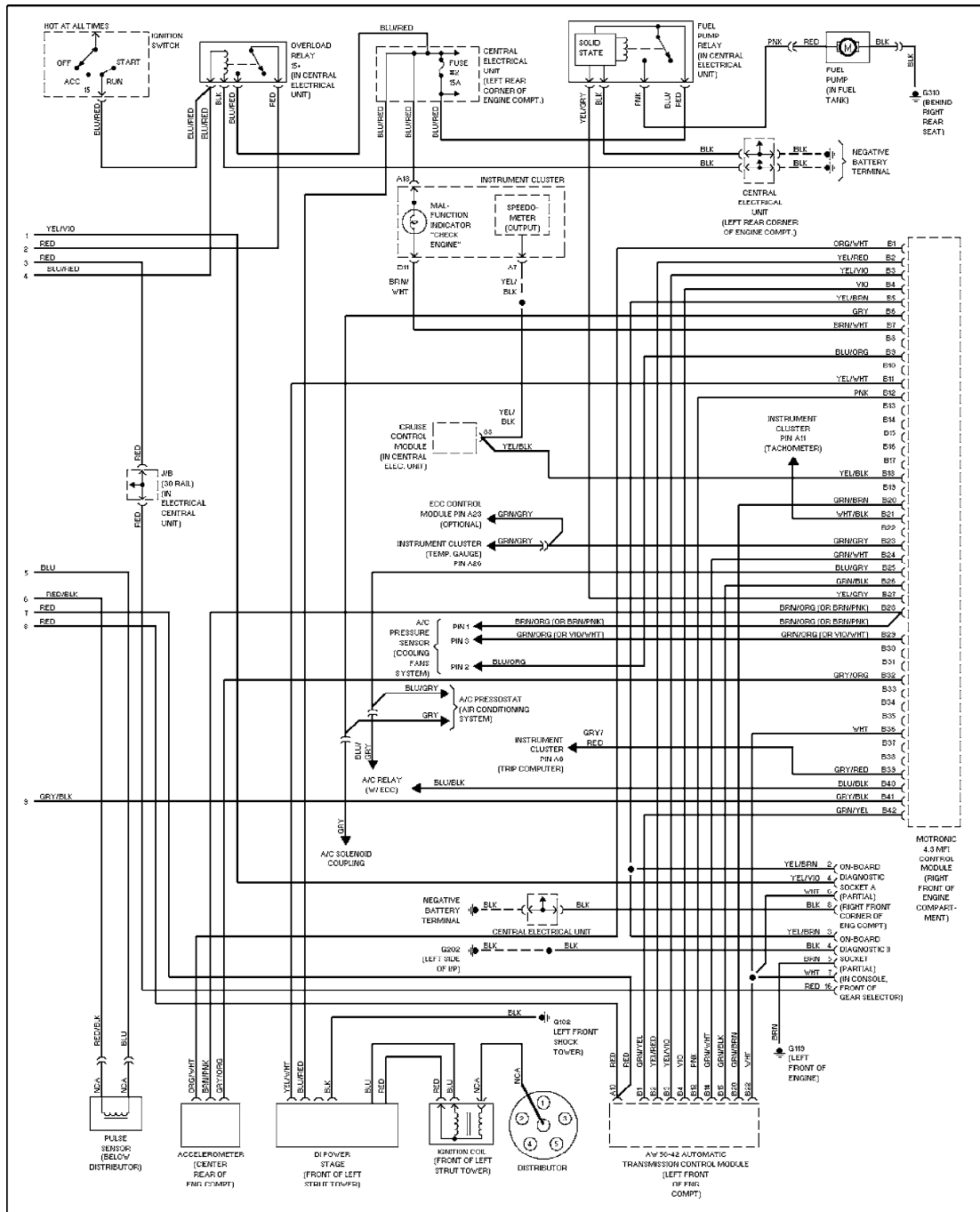
2.3L Turbo, Engine Performance Circuits (2 of 2)
