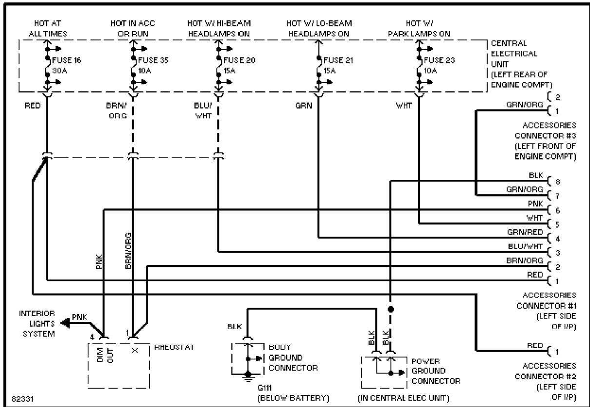
Accessories Connector Circuit, Early Production
