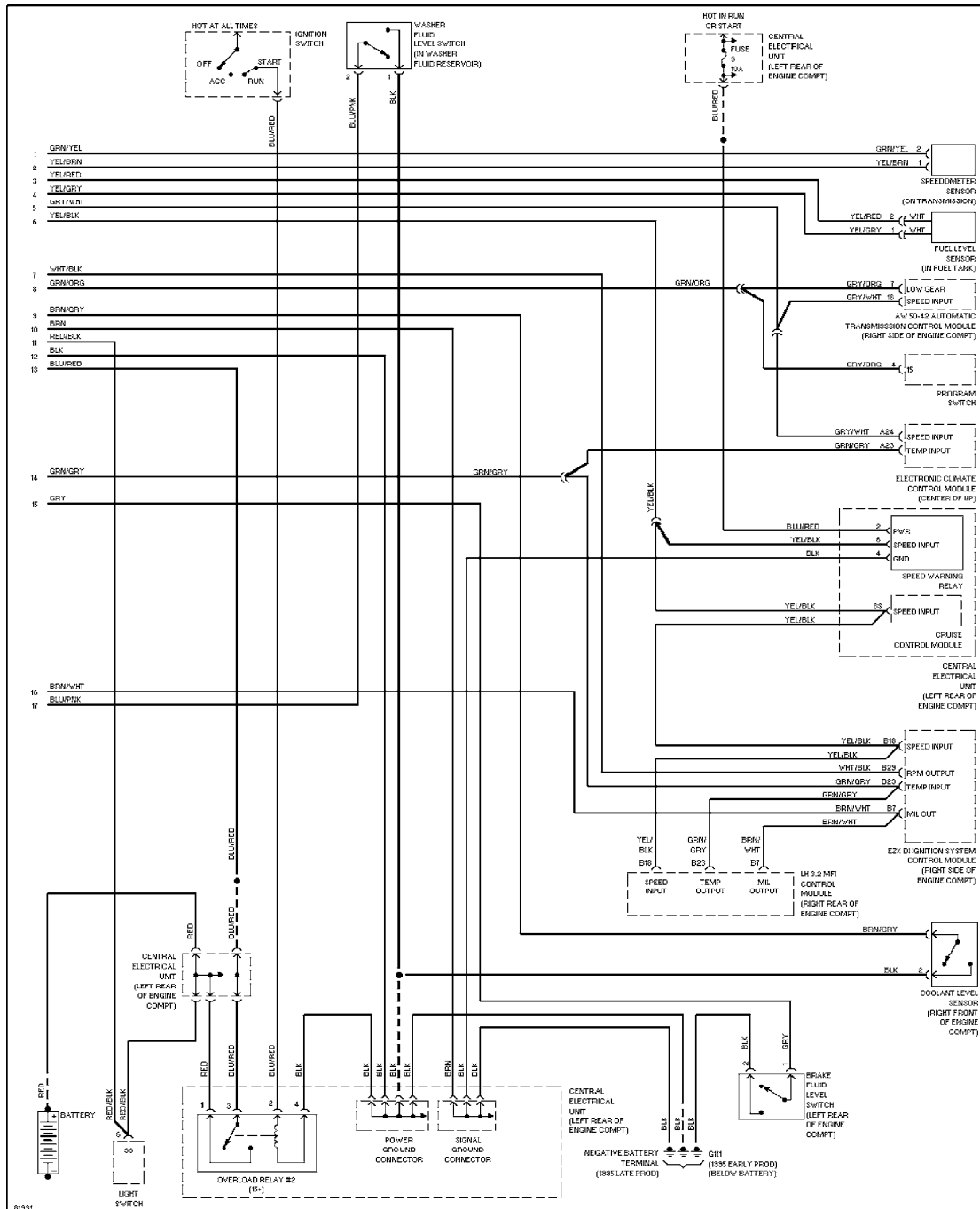
Instrument Cluster Circuit, Yasaki (2 of 2)
