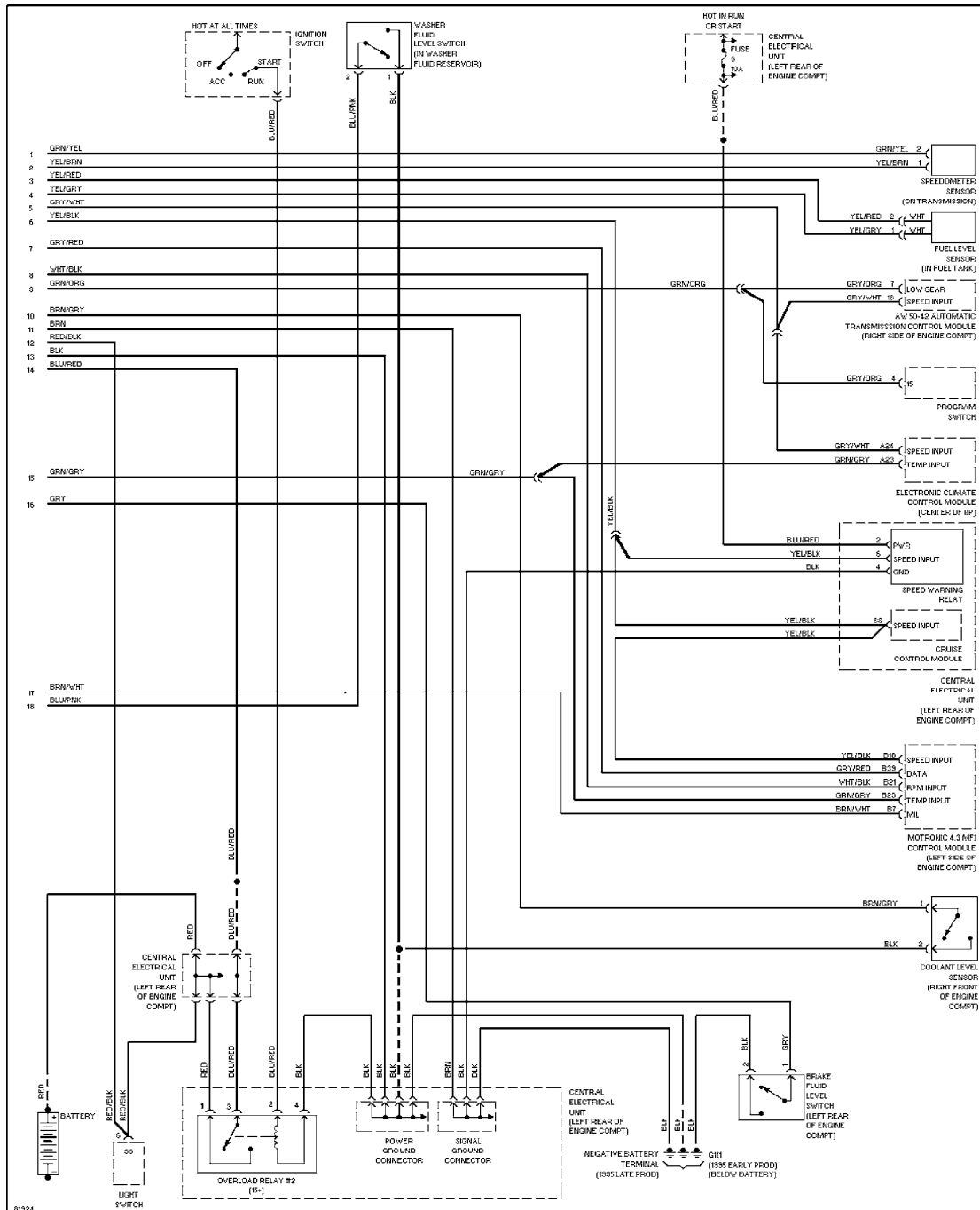
Instrument Cluster Circuit, VDO (2 of 2)
