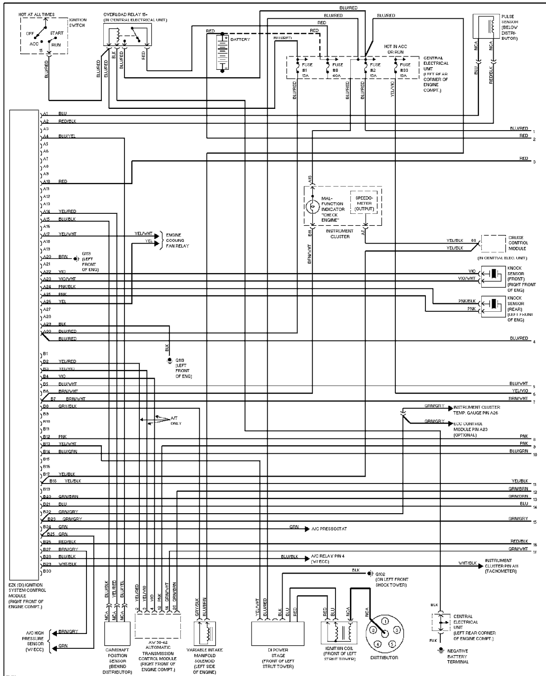
2.4L, Engine Performance Circuits (1 of 2)
