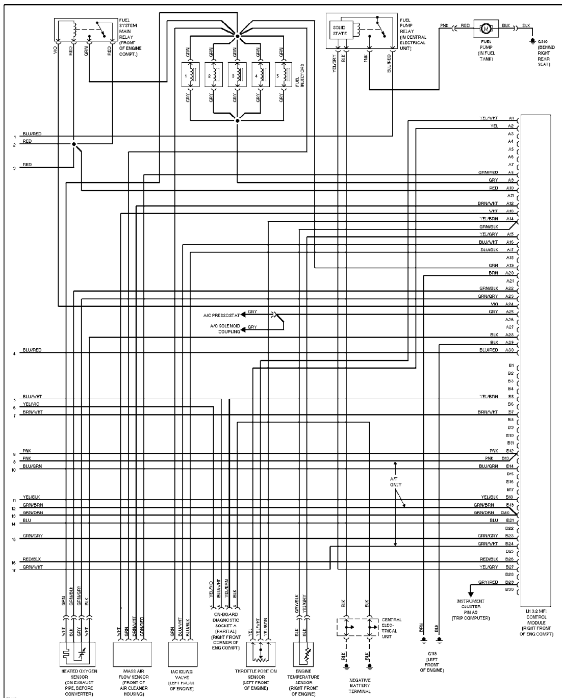
2.4L, Engine Performance Circuits (2 of 2)
