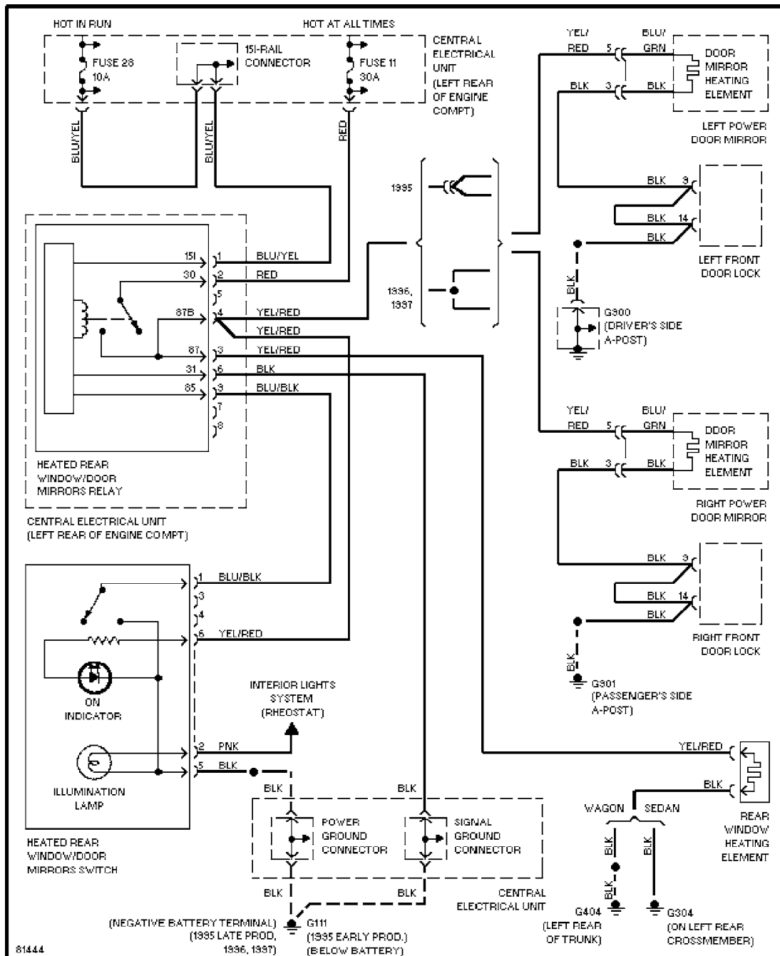
Defogger Circuit
