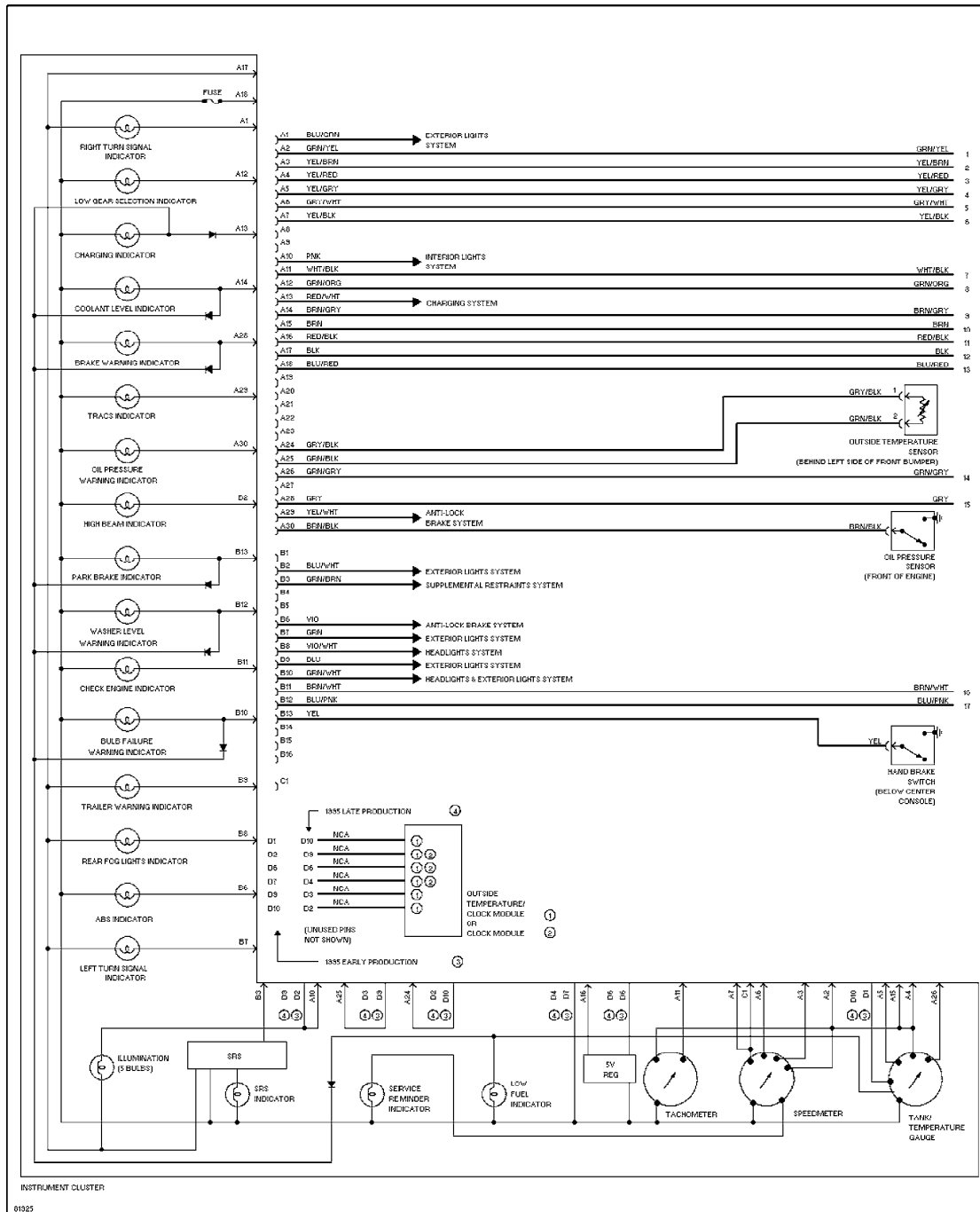
Instrument Cluster Circuit, Yasaki (1 of 2)
