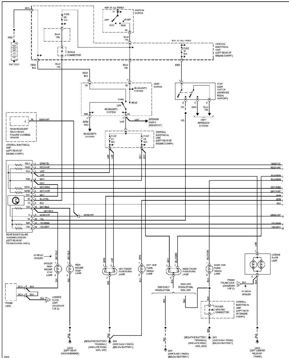
Exterior Lamps Circuit, Sedan (1 of 2)
