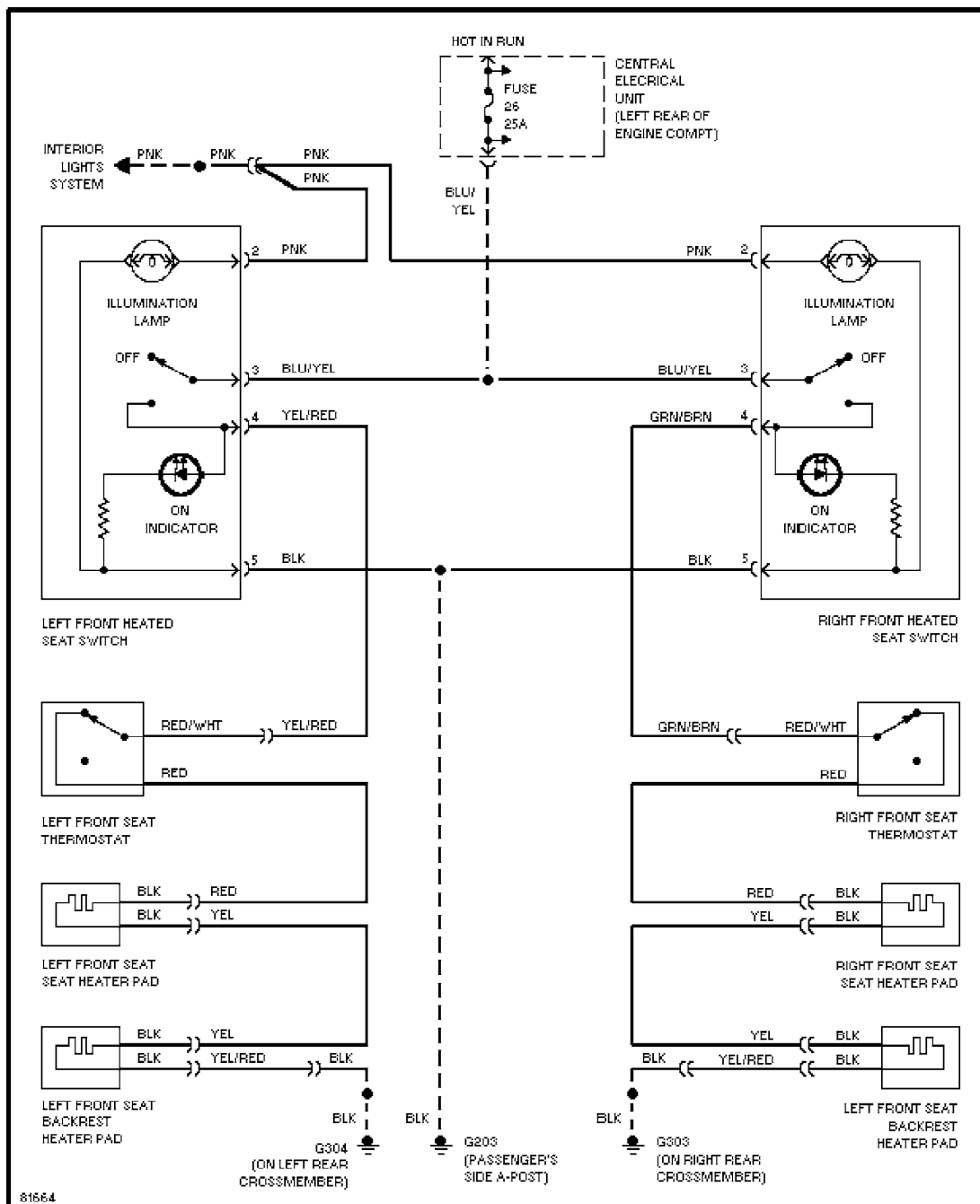
Front Seat Heater Circuit
