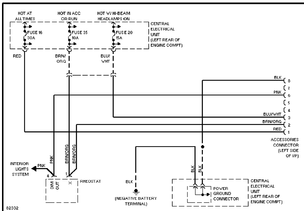
Accessories Connector Circuit, Late Production
