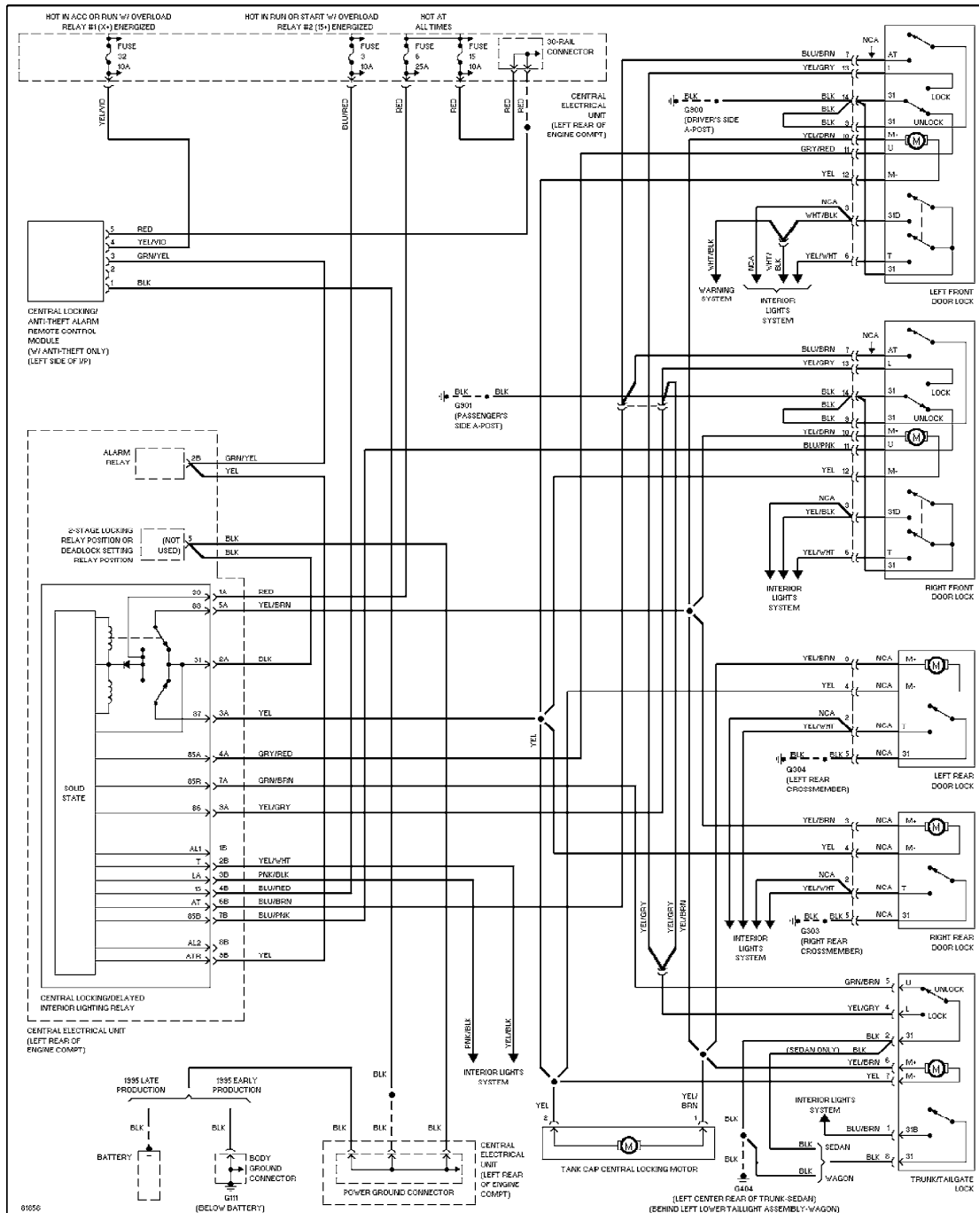
Central Locking Circuit, W/O Deadlock
