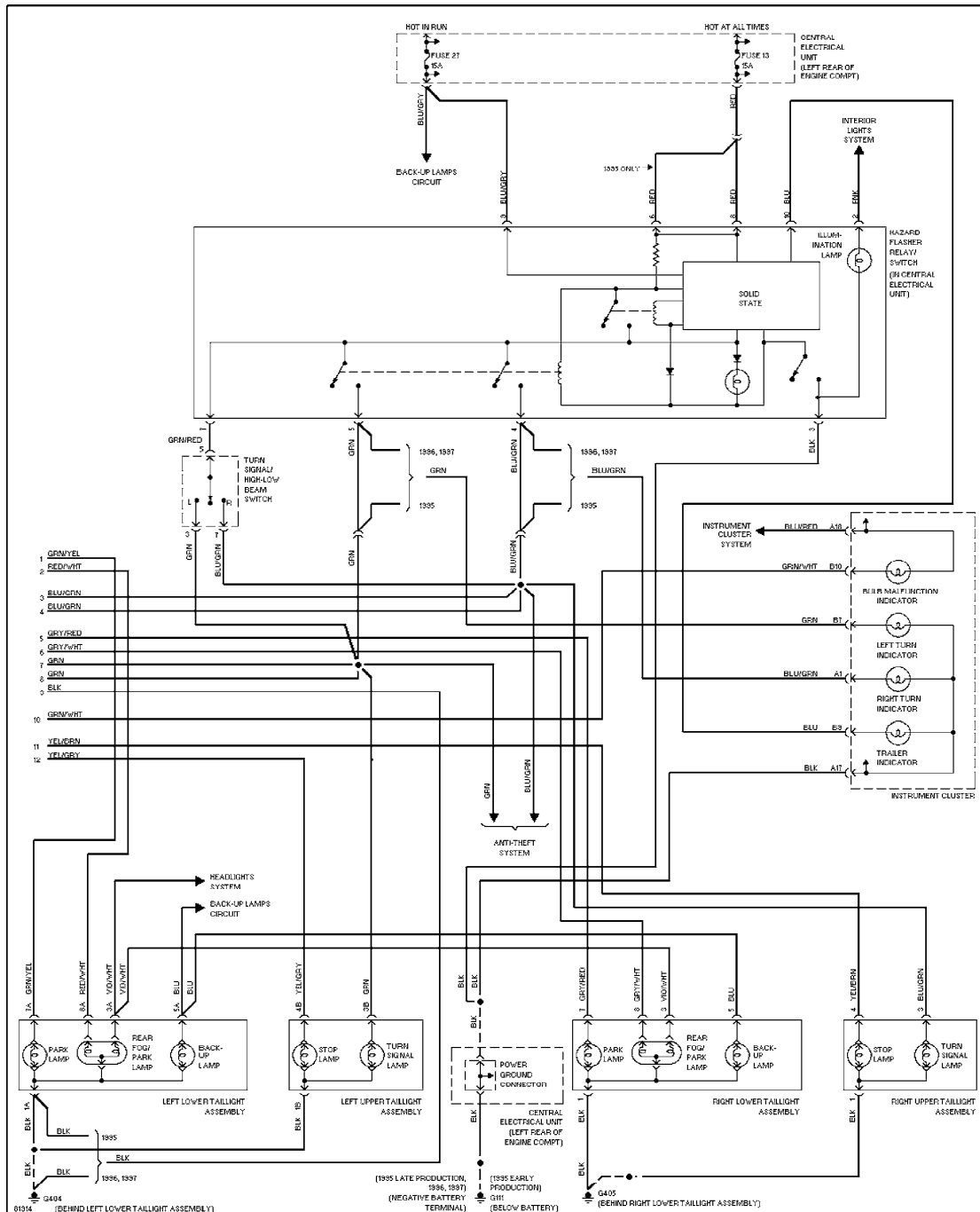
Exterior Lamps Circuit, Wagon (2 of 2)
