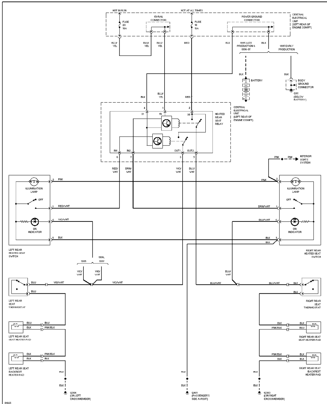
Rear Seat Heater Circuit
