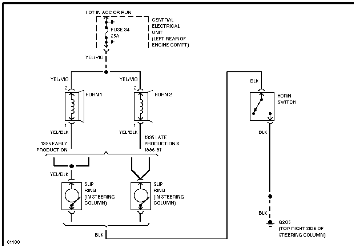
Horn Circuit
