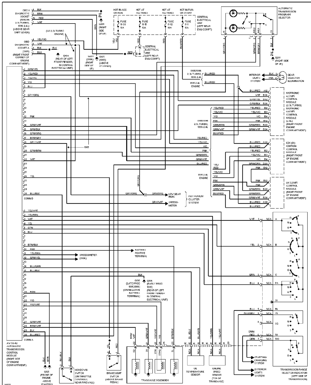
Transmission Circuit
