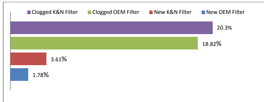
Fig 3. Percentage Resistance to Air Flow.
