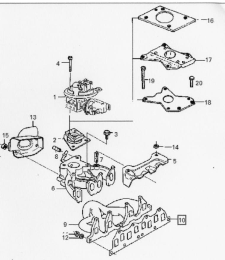
Induction and exhaust manifold valve housing. B18U. 1993-
