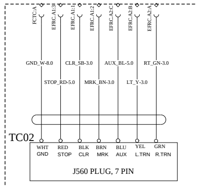
FIXED TRAILER CABLE, COILED
