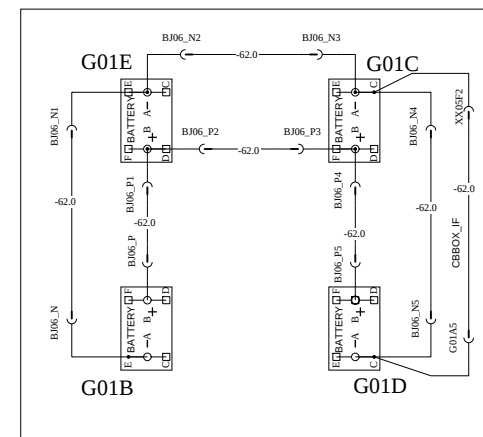
BBOX_IF CABLES FOR JUMPERS
