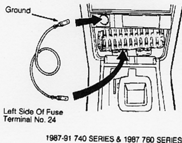
Fig. 11: Locating SRS Test Terminals (740 & 1987 760 Series) Courtesy of Volvo Cars of North America
