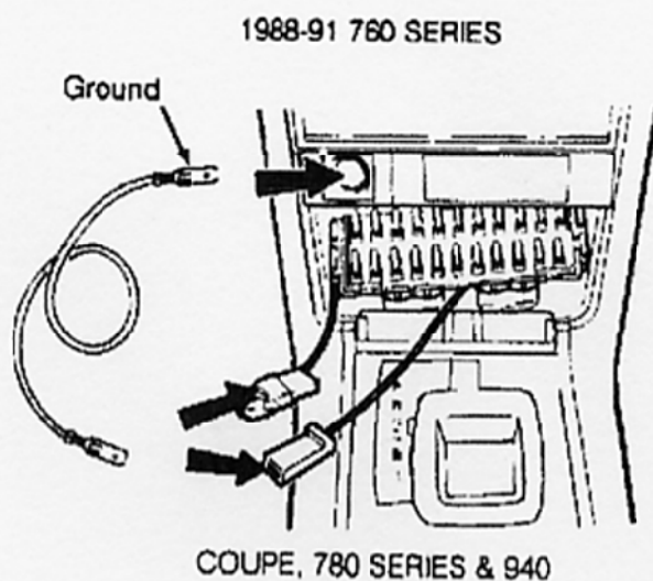
Fig. 13: Locating SRS Test Terminals (Coupe, 780 Series & 940) Courtesy of Volvo Cars of North America
