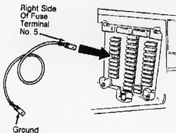
Fig. 12: Locating SRS Test Terminals (1988-91 760 Series) Courtesy of Volvo Cars of North America
